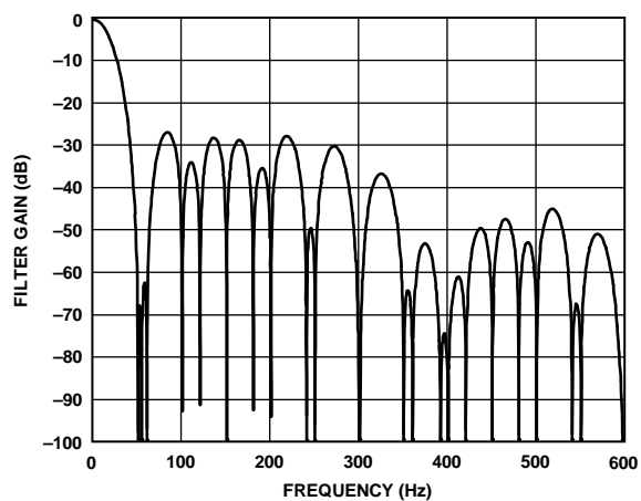
Figure 62. 25 SPS ODR, 40 ms Settling Time
