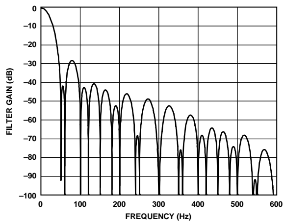
Figure 61. 27.27 SPS ODR, 36.67 ms Settling Time
