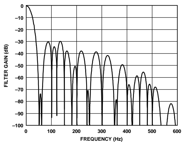
Figure 63. 20 SPS ODR, 50 ms Settling Time
