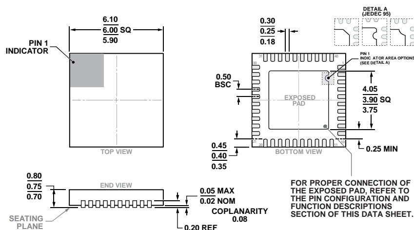
Figure 75. 40-Lead Lead Frame Chip Scale Package [LFCSP] 6 mm x 6 mm Body and 0.75 mm Package Height (CP-40-14)
